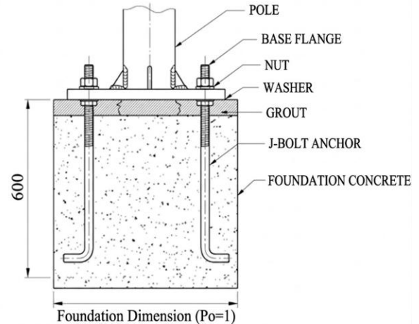
Foundation Dimension (Po=1)
