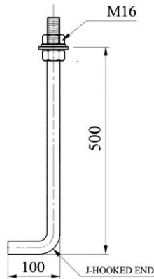
M16 J-ANCHOR BOLT ASSEMBLY DETAIL
