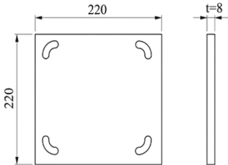
FLANGE 220x220 (t=8 mm)
