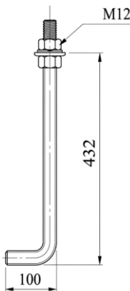
J-ANCHOR BOLT DETAIL (M12)
