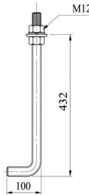
M12 J-ANCHOR BOLT ASSEMBLY DETAIL
