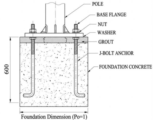
MOUNTING AND FOUNDATION DETAIL (EXAMPLE)
