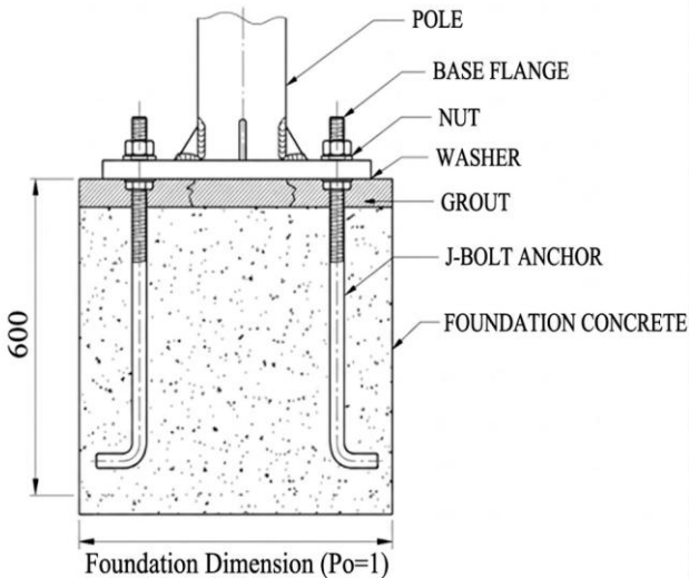
FOUNDATION DIMENSIONS (Po=1)
